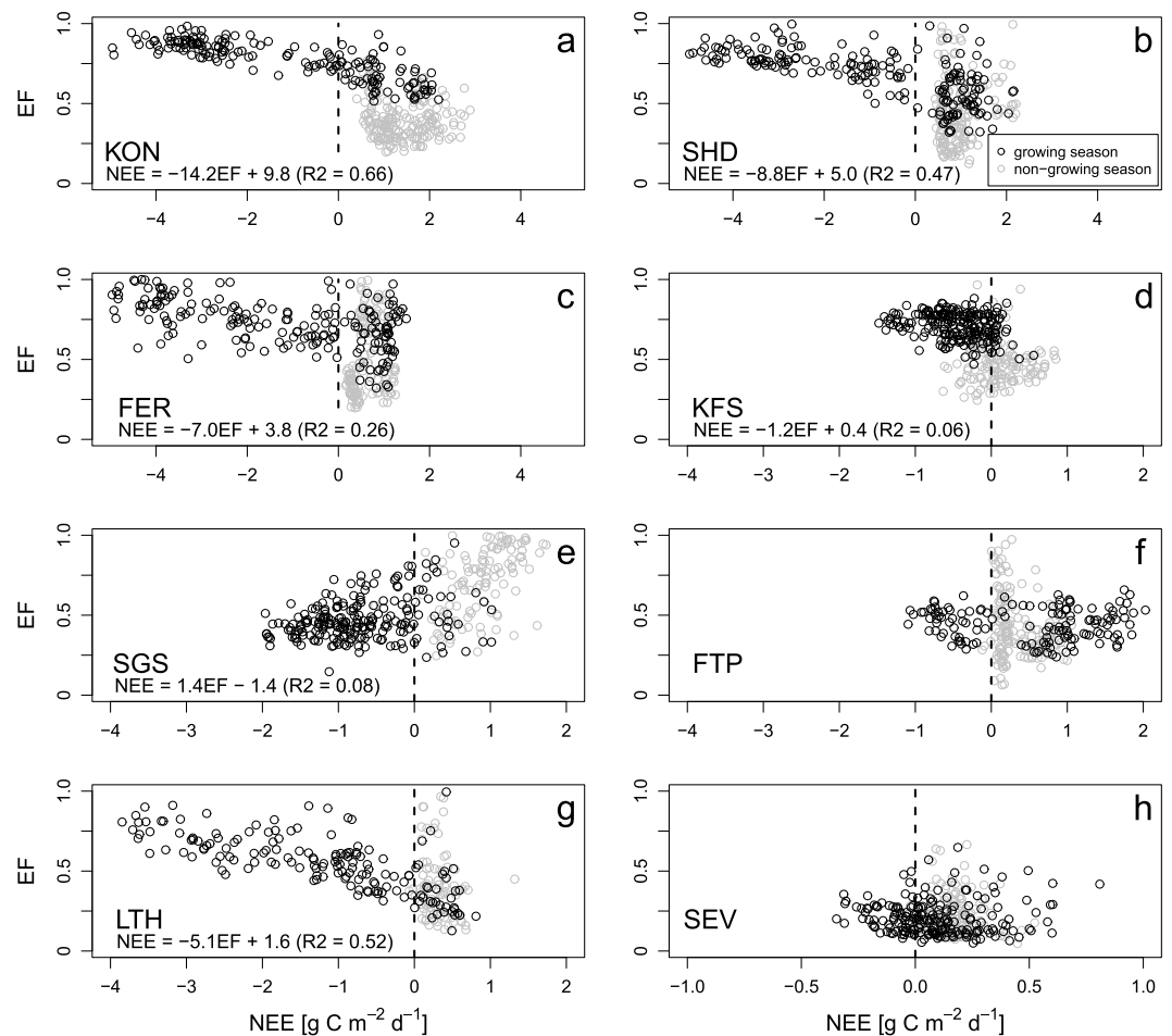
Figure 5. Relationship between daily mean net ecosystem exchange ( NEE: \text{g C m}^{-2} \text{d}^{-1} ) and daily mean evaporative fraction ( EF: \frac{LE}{H+LE} ). Points are divided between those days occurring within and outside each site's active growing season. Regression equations correspond to values during each site's active growing season. The R^2 statistic is provided in parenthesis, and all values are significant at p < 0.05 . The x axis scale differs between panels.
