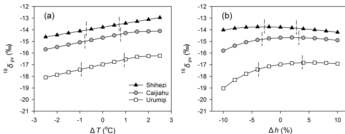
Figure 5. Variation of oxygen isotope ratios in precipitating vapor ( ^{18}\delta_{pv} ) under different conditions of temperature ( \Delta T ) and relative humidity ( \Delta h ) at Shihezi (triangle), Caijiahu (circle) and Urumqi (square). The dashed vertical lines denote the standard deviation for each line. The standard deviations of temperature and relative humidity are based on the annual average data during summer months (April–October) from 1981 to 2010.
