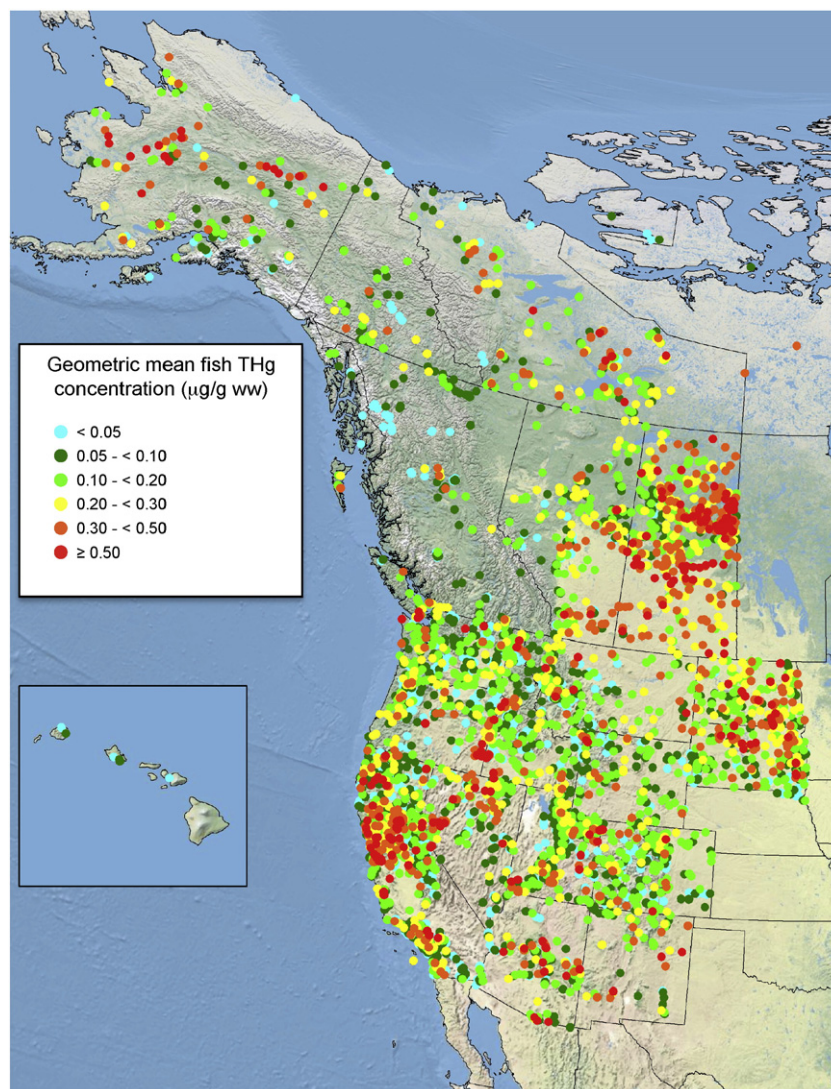
Fig. 1. Site-specific geometric mean fish total mercury (THg) concentrations ( \mu\text{g/g} wet weight) across Western US and Canada. Concentrations represent geometric mean THg in muscle tissue across all fish species and years for each site. Data are not adjusted for fish size. Sample sizes varied considerably by location. See Fig. S2 for distribution of data from sites with at least 3 individuals.
