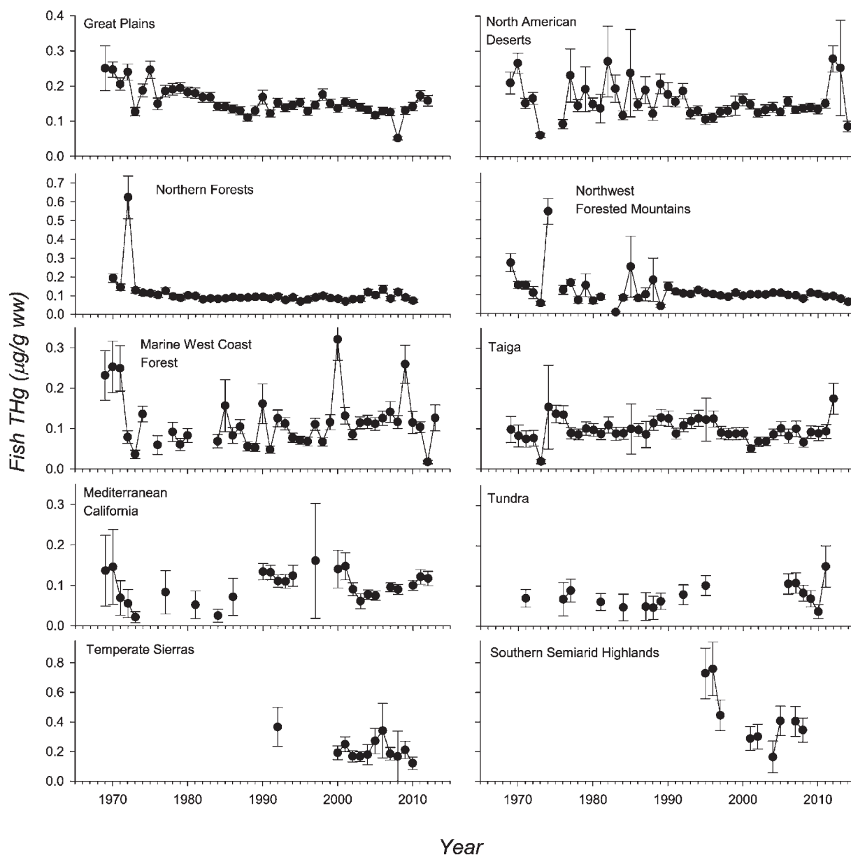
Fig. 9. Least squares mean total mercury (THg) concentrations ( \mu\text{g/g ww} ) in size-standardized fish muscle tissue from 10 different level 1 ecoregions across western North America between 1969 and 2014. Least squares mean THg concentrations account for the effects of site and species. Error bars represent standard error.
