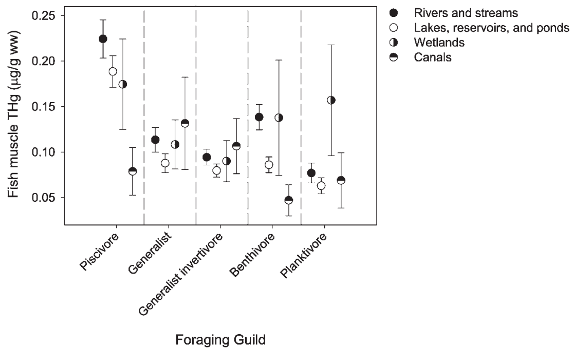
Fig. 3. Fish muscle total mercury (THg) concentrations ( \mu\text{g/g} wet weight) differ among habitat types and foraging guilds. Symbols represent size adjusted least squares (LS) mean THg concentrations controlling for the effects of species, site, and year. Error bars are one standard error.
