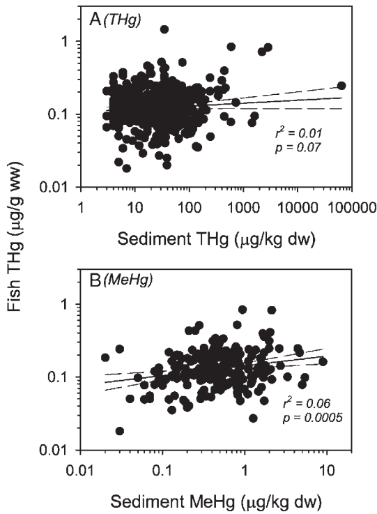
Fig. 6. Correlation between HUC-8 least squares mean fish total mercury (THg) concentrations (µg/g wet weight) and paired HUC-8 least squares mean (A) sediment THg concentrations and (B) sediment MeHg concentrations. Fish least squares mean concentrations were estimated using size standardized fish THg data in a linear mixed-effects model that included Level 1 ecoregion and HUC-8 (nested within ecoregion) as fixed effects, and site, species, and year as random effects. Sediment least squares mean concentrations were estimated from linear mixed effects models that included HUC-8 as a fixed effect, and site as a random effect (Fleck et al., in press).
