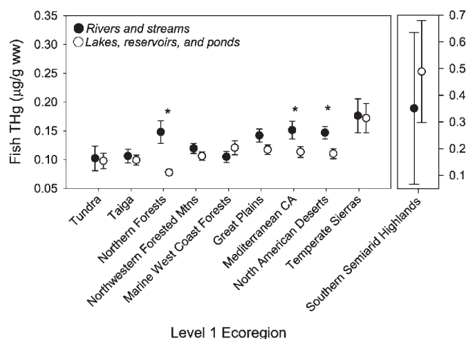
Fig. 8. Least squares mean fish muscle total mercury (THg) concentrations ( \mu\text{g/g} ww) among Level 1 ecoregions for rivers and streams (black circles) and lakes, ponds, and reservoirs (white circles). Least squares mean THg concentrations were estimated using length-standardized THg concentrations in a linear mixed effects model that included habitat and level 1 ecoregion as fixed effects, and site, species, and year as random effects. Error bars represent standard error. * indicates statistical differences ( \alpha = 0.05 ) between lentic and lotic habitats within ecoregions. Note the difference in y-axis scale for Southern Semiarid Highlands relative to the other ecoregions.
