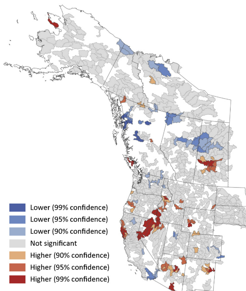
Fig. 5. Analysis of fish total mercury concentration “hotspots” and “coldspots” at the HUC-8 watershed scale across western North America. Watersheds shaded red and blue represent least squares mean fish THg concentrations that are higher or lower, respectively, than expected by chance alone based upon adjacent watersheds. Different shades of red and blue represents different levels of statistical confidence. Spatial autocorrelation and statistical significance was determined using the Getis-Ord G_i^* statistic.
