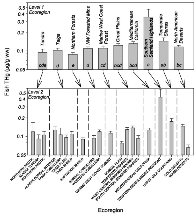
Fig. 7. Least squares mean fish THg concentrations (µg/g ww) across Level 1 (top panel) and Level 2 (bottom panel) ecoregions in the western US and Canada. Least squares mean THg concentrations were estimated using length-standardized fish muscle THg concentrations in a linear mixed effect model that included Level 1 and Level 2 (nested within Level 1) ecoregions, and HUC-8 (nested within ecoregion) as fixed effects, and site, species, and year as random effects. Error bars represent 1 standard error. Different letters represent statistical significance (alpha = 0.05) determined using Tukey's pairwise differences.
