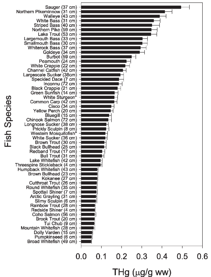
Fig. 2. Least squares mean, size standardized muscle tissue total mercury (THg) concentrations ( \mu\text{g/g} wet weight) in fish species across western US and Canada. Data represent species with a total sample size of > 100 individuals. Error bars represent 1 standard error. Least squares mean concentrations represent the mean THg concentration in each species after controlling for site and year effects. Fish THg concentrations were standardized to the respective median length for each species, shown in parentheses. * indicates there weren't length-THg relationships and THg concentrations are not size-standardized.
