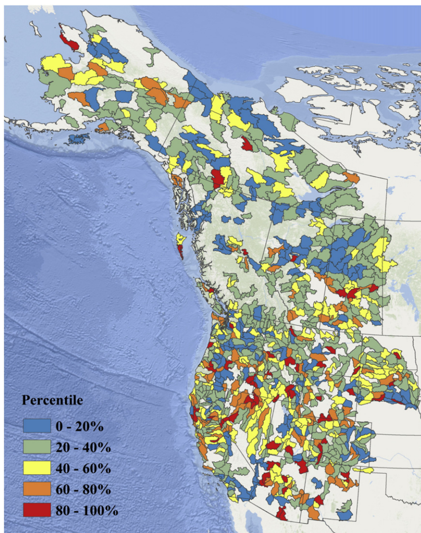
Fig. 4. Relativized total mercury (THg) concentrations (binned by quintiles of the data distribution) in fish across the western United States and Canada. Each bounded polygon represents a hydrologic unit at the HUC-8 scale. The categories represent the percentile of least squares mean THg concentration relative to the entire dataset, such that 20% of the data distribution occurs in each HUC. The least squares mean THg concentrations in the lowest category (0–20th percentile) ranged between 0.011 and 0.074 \mu\text{g/g} ww. The least squares mean THg concentrations in the 20th–40th percentile ranged between 0.075 and 0.126 \mu\text{g/g} ww. The least squares mean THg concentrations in the 40th–60th percentile category ranged between 0.127 and 0.178 \mu\text{g/g} ww. The least squares mean THg concentrations in the 60th–80th percentile category ranged between 0.179 and 0.248 \mu\text{g/g} ww, and the least squares mean THg concentrations in the highest category (80th–100th percentile) ranged between 0.249 and 1.45 \mu\text{g/g} ww. Least squares mean THg concentrations were estimated from a linear mixed effects model with level 1 ecoregion and HUC-8 (nested within ecoregion) as fixed effects, and species, site, and year as random effects. HUC-specific sample size and coefficient of variation are presented in Fig. S5.
