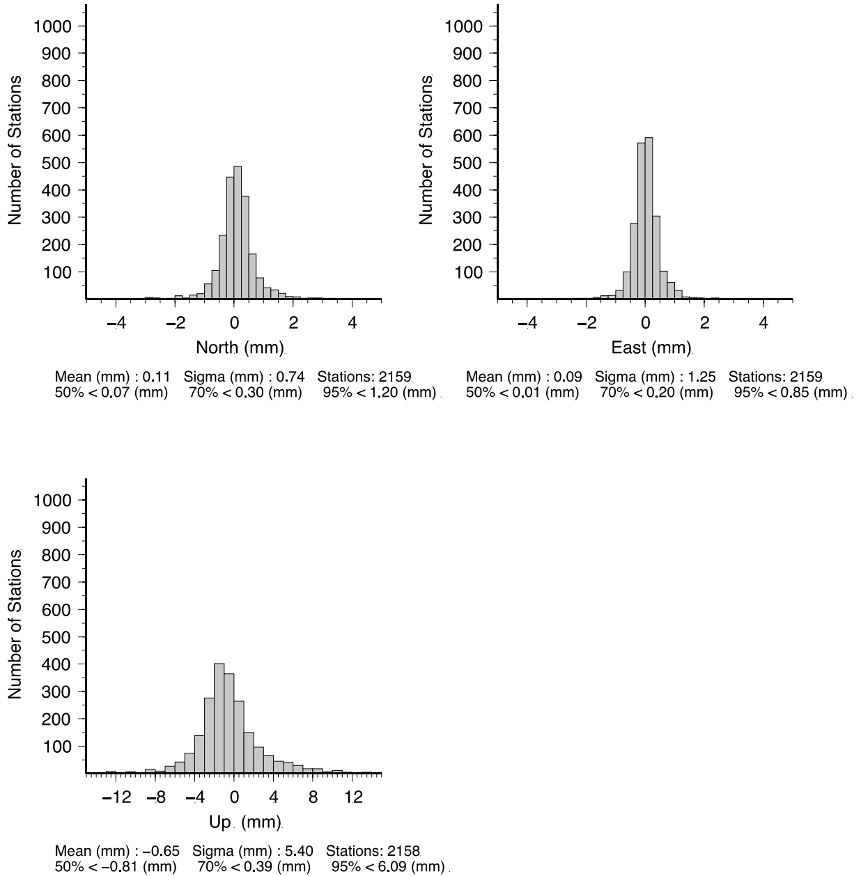
Figure 5. Histograms of the mean position differences between NMT and CWU analysis. These histograms are generated by differencing the time series for each station and finding the weighted mean of the differences. The sense here is NMT-CWU.
