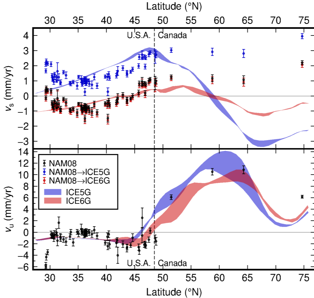
Figure 17. Southward (top) and vertical (bottom) velocities plotted as a function of latitude along a 5000 km profile from site RESO (Resolute Bay) in Canada (right) to the Gulf of Mexico near LMCN and GRIS (left). The Canadian stations are RESO, BAKE, CHUR and PICL. The width of the profile is ~1500 km and covers a box with longitude and latitude coordinates of 261.7156, 75.4857; 267.4151, 75.7914; 267.0573, 27.4141 and 272.7568, 27.7198 (deg). The profile is shown on the maps in Figure 16. The vertical profile clearly shows the collapse of the peripheral bulge (~45° latitude) related to GIA. The vertical rates at the end of the profile (latitude <30°) are mostly likely local to the Houston area and therefore not representative of GIA. The solid envelopes are from the ICE6G (red) and ICE5G (blue) GIA models, both of which have been tuned to match the vertical GPS motions. The circles with error bars are the GAGE NAM08 estimates (black) and these same estimates with a North America Euler pole estimated to best match the GIA horizontal motion estimates (blue for ICE5G, red for ICE6G). ICE5G and ICE6G results interpolated from the gridded velocity estimates available at http://www.atmosph.physics.utoronto.ca/~peltier/data.php . [Peltier, 2004; Peltier et al. , 2015]. The envelopes represent the ranges of the models within the width of the profile, not the uncertainties.
