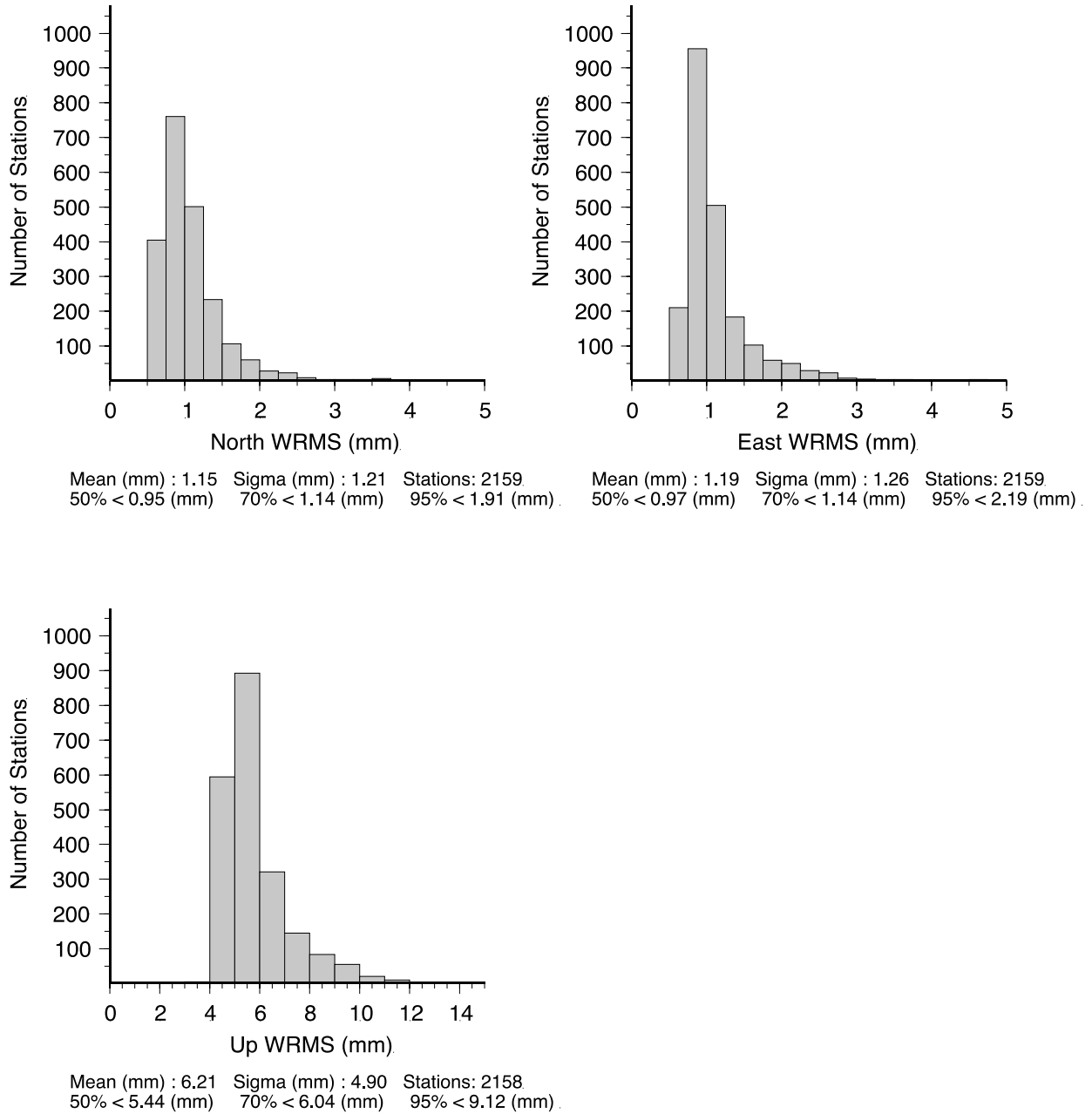
Figure 7. Histograms of the WRMS scatters of the differences between the positions estimates from the CWU and NMT analyses.
