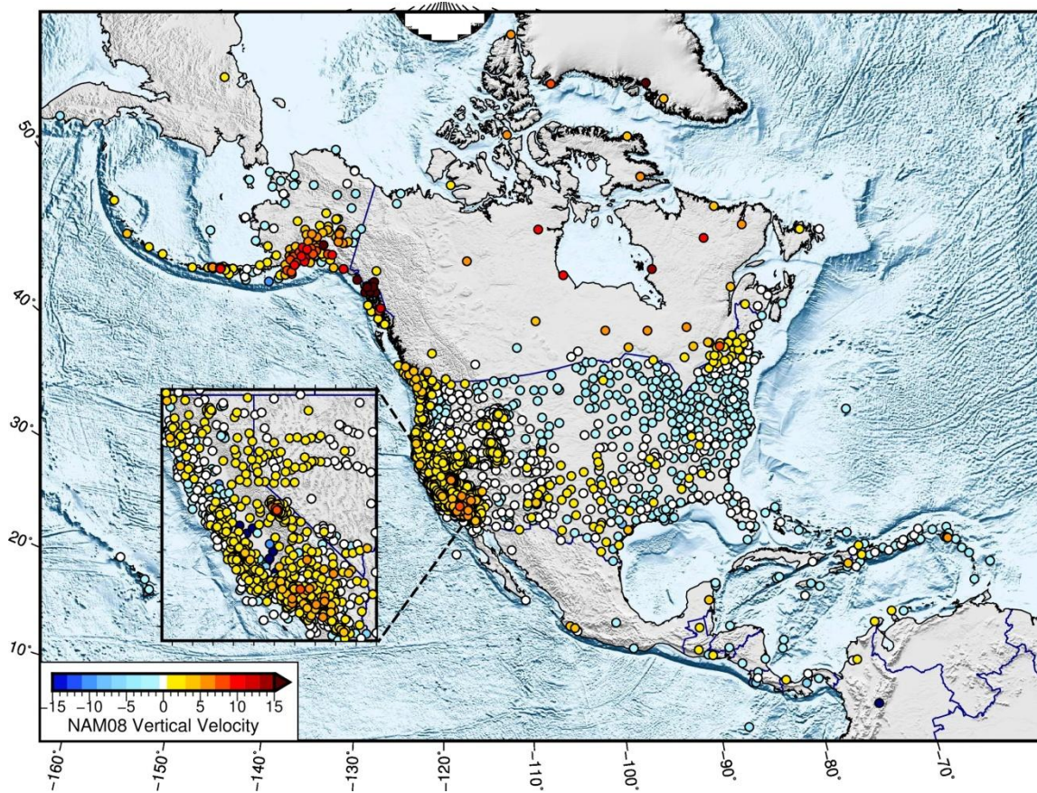
Figure 14. Geographic distribution of vertical velocities. Only those stations with vertical velocities with uncertainties < 2 mm/yr are shown. Note the generally negative vertical velocities in the midwest and eastern part of the US and the generally positive vertical velocities in the western US, with southern CA showing some of the highest positive values.
