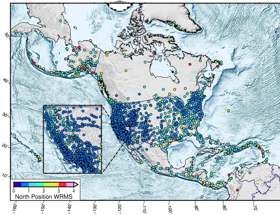
Figure 9. WRMS scatter of the north position residuals (mm) after removing linear trends, offsets, annual sine and cosine terms, and in some case post-seismic logarithmic terms. There are 2137 stations shown and the values are based on GAGE analysis from 1996 to 2015.
