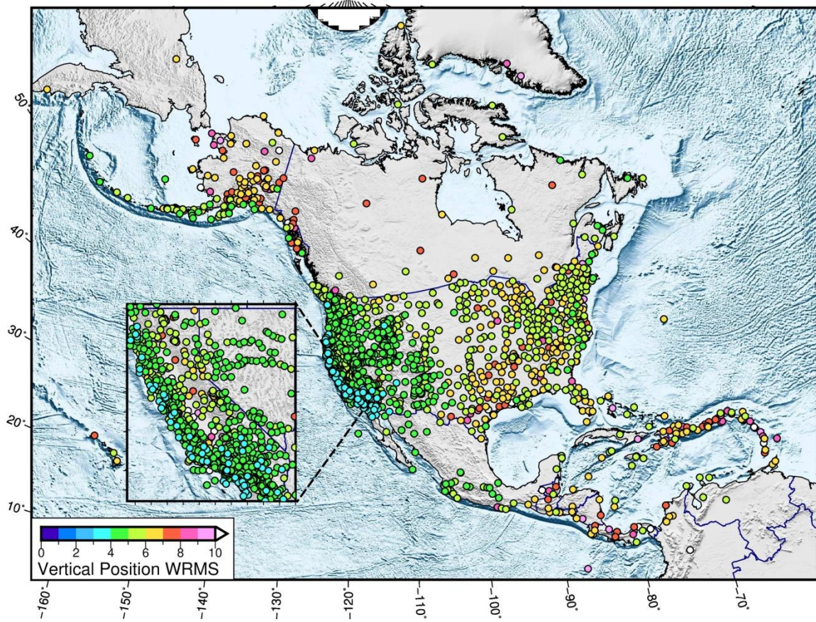
Figure 11. WRMS scatter of the height position residuals (mm) after removing linear trends, offsets, annual sine and cosine terms, and in some case post-seismic logarithmic terms. The scale used here is larger than that in Figure 4.2.2, reflecting the larger uncertainty in height.
