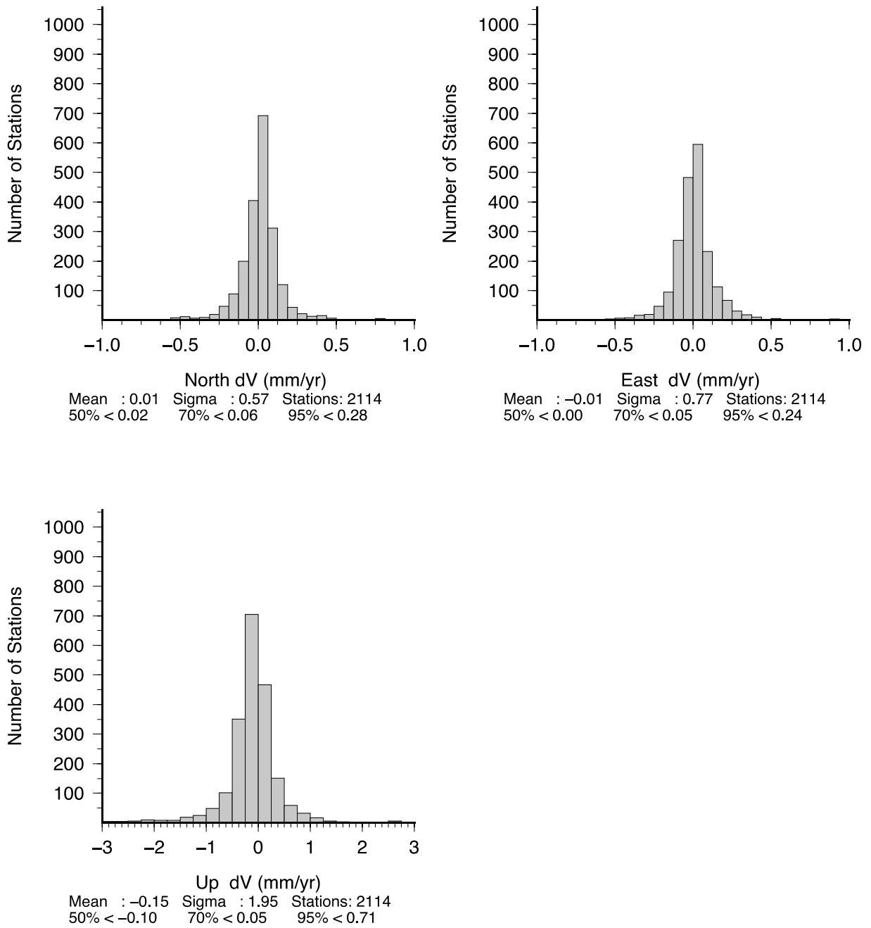
Figure 4. Histograms of the differences in velocity estimates between the NMT and CWU analyses. The mean vertical rate difference is not equal to the value in Table 4 because the value in Table 4 is a weighted mean difference, whereas here it is an arithmetic mean.
