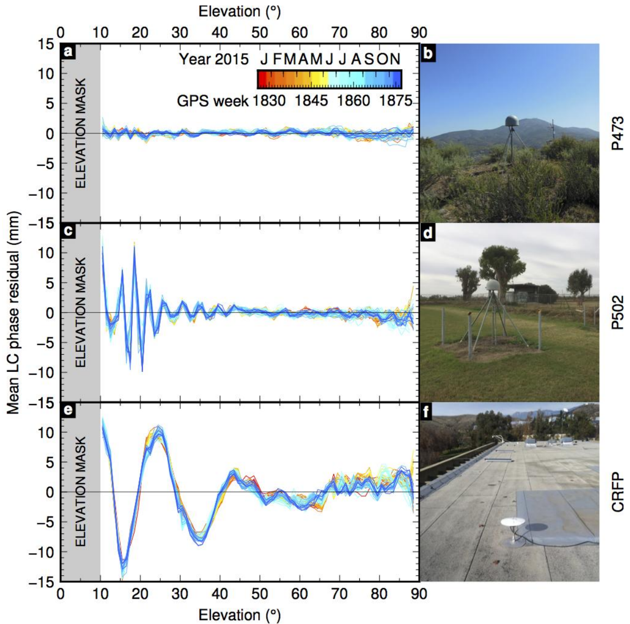
Figure 13. Mean ionosphere-free phase residuals for all satellites, averaged over each week of 2015 in 1^\circ elevation angle bins above the horizon, and photographs of the antennas for: (a,b) a station with a good scattering environment, P473; (c,d) a station with some multipath from a grassy plane, P502; and (e,f) a station in a poor signal reflection environment, CRFP, whose antenna is mounted near a metal covering on a roof, as shown in (f), resulting in large multipath effects at low elevation angles. The color scale for (c) and (e) is the same as shown in (a).
