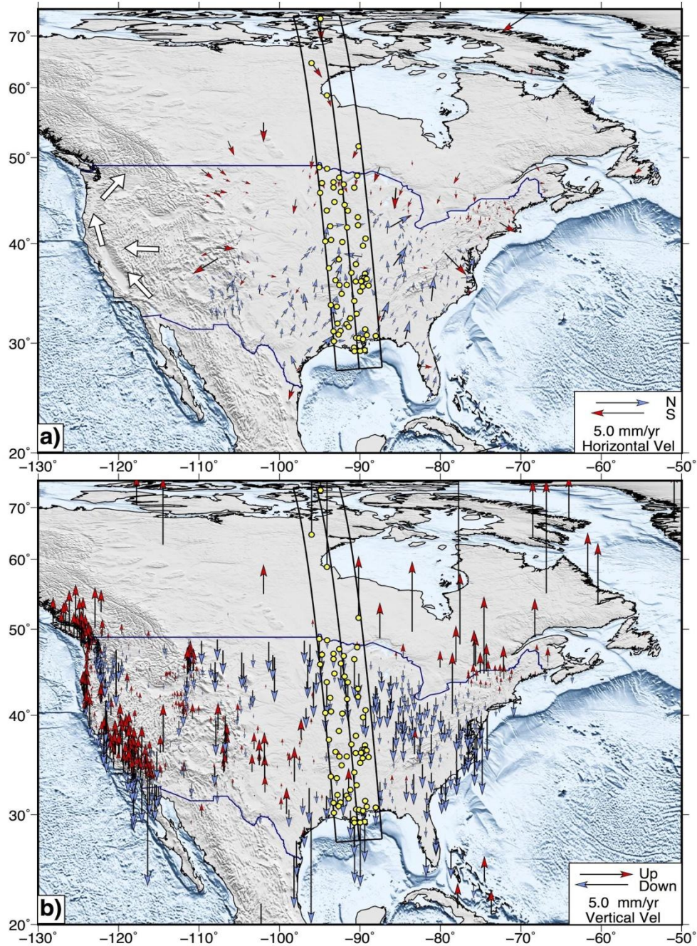
Figure 16. Map of stations used to estimate GIA effects (nearly NS profile) in cylindrical projection. Subplots show a) horizontal velocities and b) vertical velocities. Arrowheads are color-coded to indicate whether a station has north (blue) vs south (red) motion, and uplift (red) vs. subsidence (blue). Error ellipses/bars shown in the legend are 2-sigma, but error ellipses are not shown on the map for clarity. Only those stations with horizontal errors <0.5 mm/yr in both the north and east components are plotted. The more densely instrumented and faster moving stations east of 110^{\circ}\text{W} are not shown in subplot (a). Instead the general sense of motion in the western US is represented by the white arrows.
