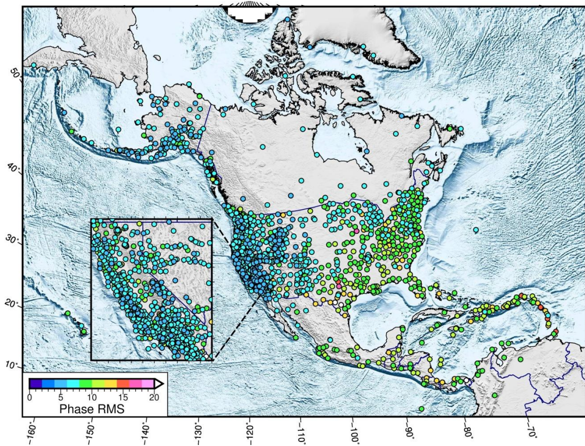
Figure 8. Average root-mean-square (RMS) scatter of the phase residuals in mm for 1969 stations from which data are available during the period from 2014/11/23 to 2016/02/28.
