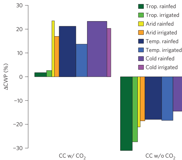
Figure 2 | Simulated CWP responses across agro-climatic regions. The median change in rainfed and irrigated CWP (%) in tropical (trop.), arid, temperate (temp.) and cold regions simulated under RCP 8.5 by 2080 relative to 2000 for all crops—GGCMs—GCMs combinations for CC w/ CO 2 and CC w/o CO 2 only. The width of the boxes varies according to corresponding total crop irrigated and rainfed harvested areas.
