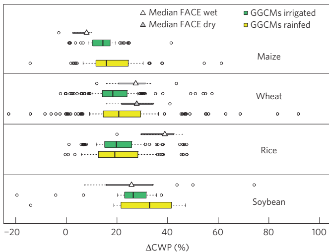
Figure 1 | Comparison between FACE observations and GGCM simulations. CWP responses to elevated [\text{CO}_2] (550 ppm from FACE and corresponding grid-cell values extracted from GGCM simulations in this study) for maize, wheat, rice and soybean at ample and limited soil water. FACE data were collected from references summarized in Supplementary Table 1. The left and right sides of the boxes are lower and upper quartiles, respectively, and the band near the middle of the boxes is the median value across each set of simulations. Open circles are outliers. Note rainfed simulations for maize and rice at the FACE locations correspond to negligible water stress conditions.
