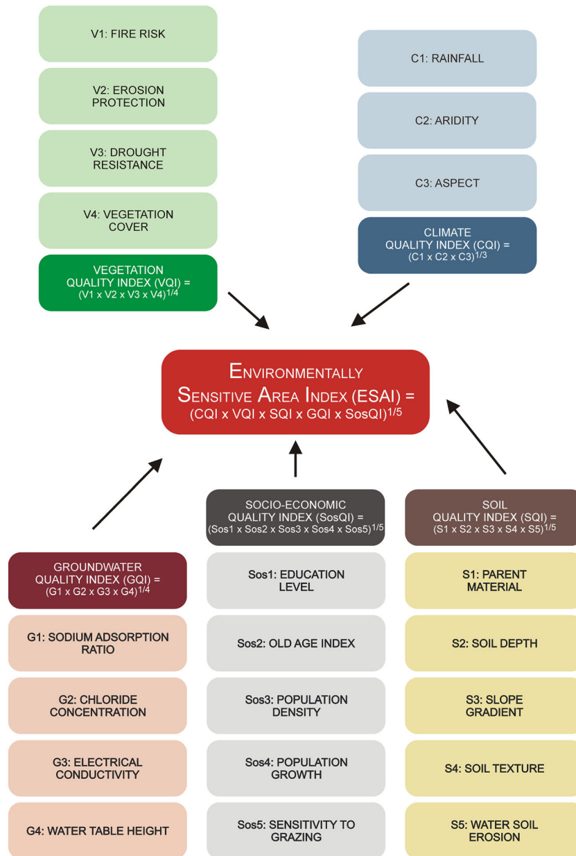
Figure 2. Flowchart of the methodological framework for the estimation of the modified Environmentally Sensitive Area Index (ESAI). This figure is available in colour online at wileyonlinelibrary.com/journal/ldr
