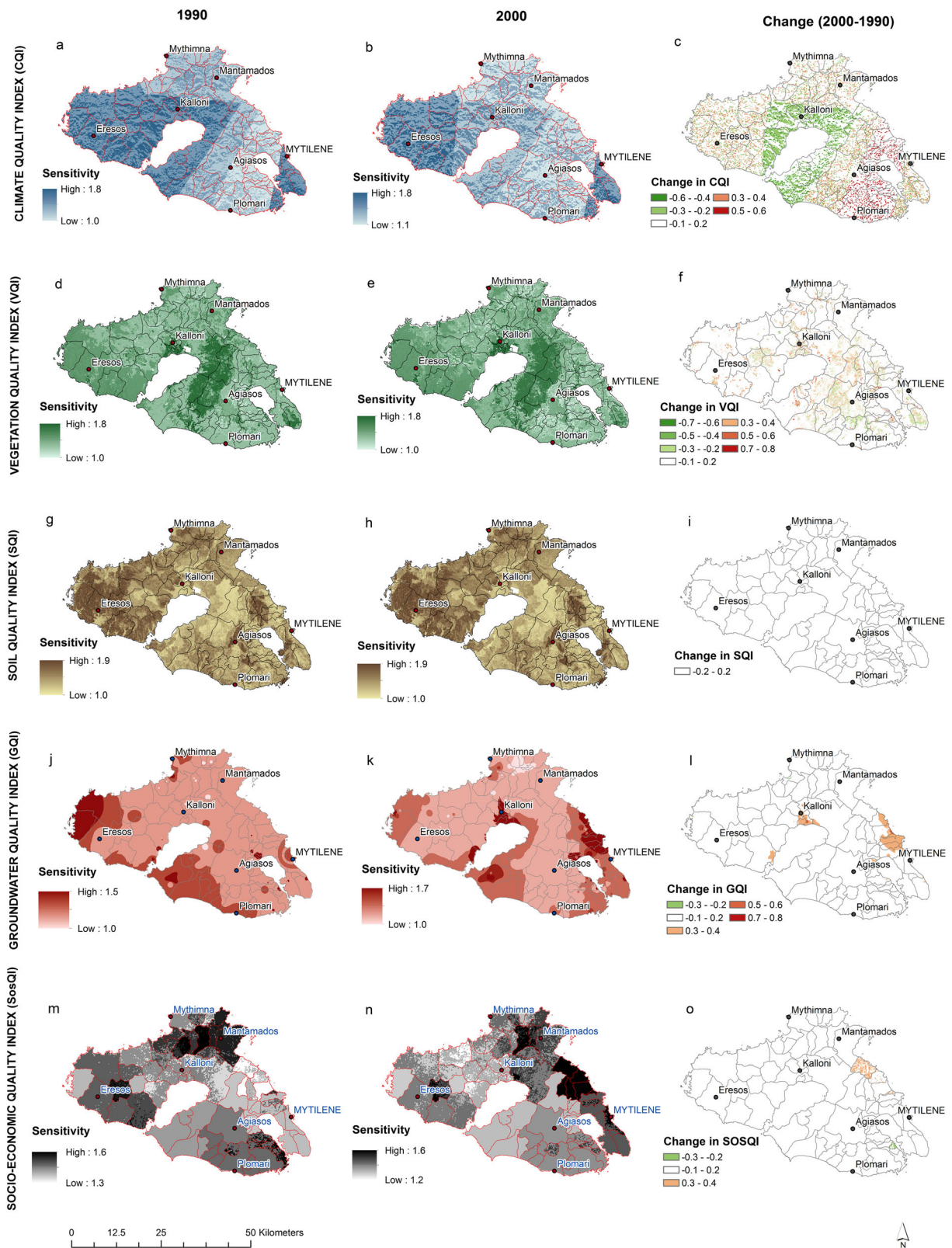
Figure 3. Sensitivity maps for 1990 and 2000 and respective change: (a), (b) and (c) Climate Quality Index (CQI); (d), (e) and (f) Vegetation Quality Index (VQI); (g), (h) and (i) Soil Quality Index (SQI); (j), (k) and (l) Groundwater Quality Index (GQI); (m), (n) and (o) Socio-economic Quality Index (SosQI). This figure is available in colour online at wileyonlinelibrary.com/journal/ldr
