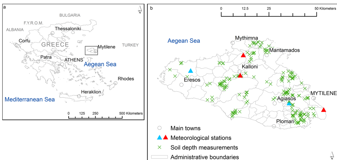
Figure 1. (a) The location of the study area, the island of Lesvos, in the Aegean Sea, Greece. (b) Locations of meteorological stations, soil depth field measurements, main localities and administrative sub-municipal boundaries. The subset of red stations are the ones used for the estimation of potential evapotranspiration. This figure is available in colour online at wileyonlinelibrary.com/journal/ldr
