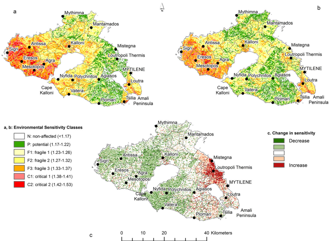
Figure 4. Environmental sensitivity according to the Environmentally Sensitive Area Index for (a) 1990 and (b) 2000. (c) Change in sensitivity between 1990 and 2000. This figure is available in colour online at wileyonlinelibrary.com/journal/ldr
