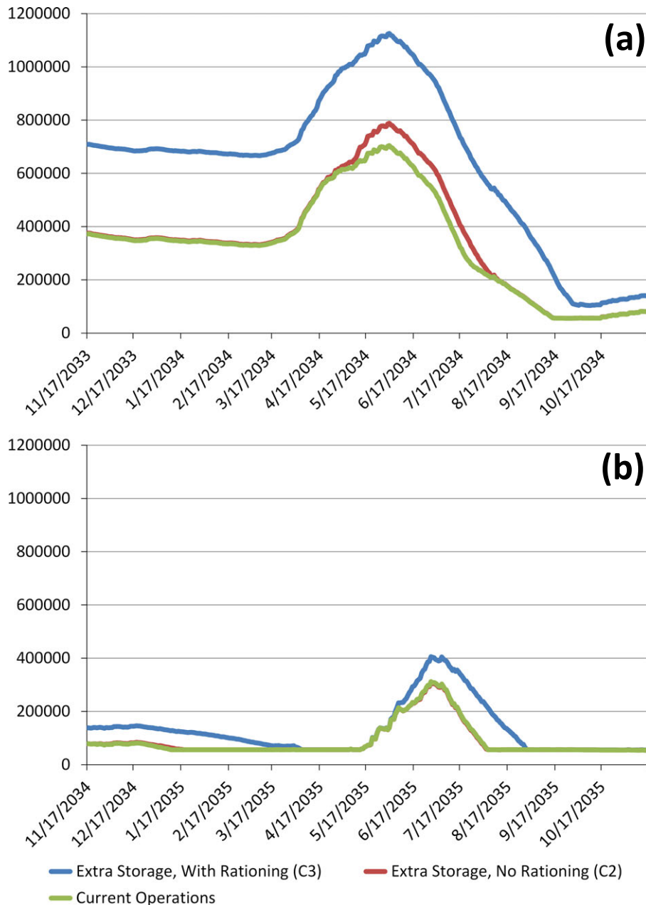
FIGURE 9. OASIS Modeled Daily Storage (dam 3 ) in the Three Alberta Environment and Sustainable Resource Development (AESRD) and Chin Reservoirs for the 2-year Min Hydroclimatic Scenario for the (a) First Year and (b) Second Year of the Projected 2033-2034 Drought, Using the C2 and C3 Adaptation Strategies.
