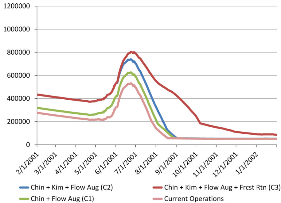
FIGURE 11. OASIS Modelled Daily Storage (dam 3 ) in the Three Alberta Environment and Sustainable Resource Development (AESRD) and Chin Reservoirs for the Observed Drought of 2001-2002, Using the C3, C2, and C1 Adaptation Strategies and Current Operations.
