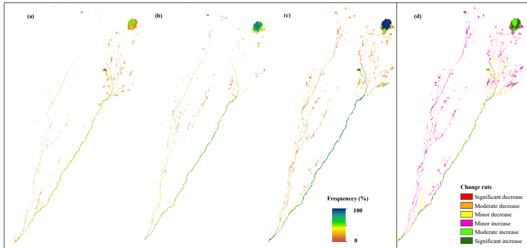
Figure 6. Frequency of inundation for (a) period 1 (1988–1998), (b) period 2 (2000–2007) and (c) period 3 (2008–2015); (d) the change rate between periods 1 and 3.
