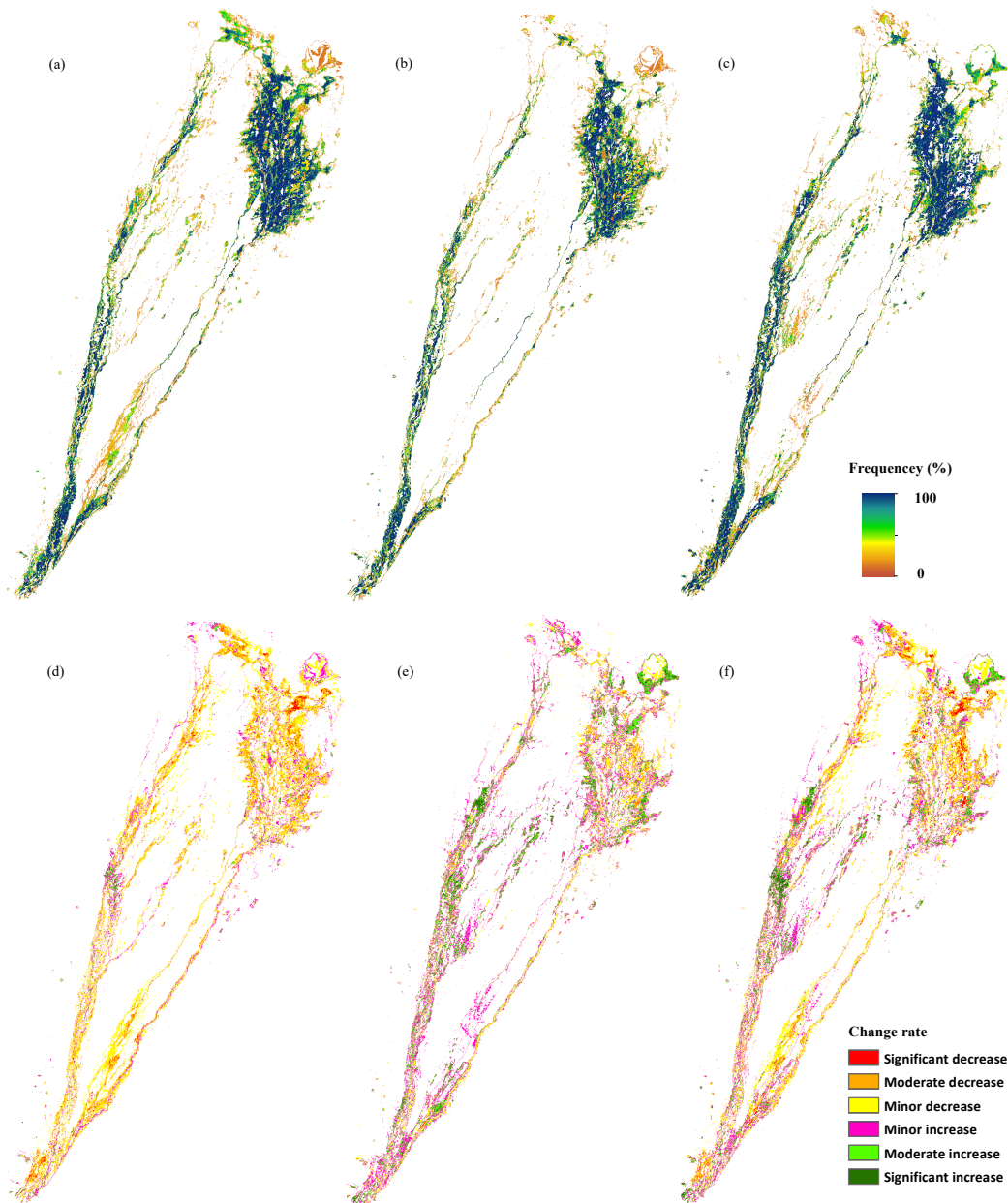
Figure 5. Spatial distribution of vegetation-covered regions in Ejina Oasis. The upper row shows the frequency of vegetation distribution for the three periods: (a) period 1 (1988–1998, no data were available for 1989 and 1997, data for 1993 were excluded for their poor quality), (b) period 2 (2000–2007) and (c) period 3 (2008–2015). The lower row shows the corresponding changes between the pairs of periods: (d) changes between periods 1 and 2, (e) changes between periods 2 and 3 and (f) changes between periods 1 and 3.
