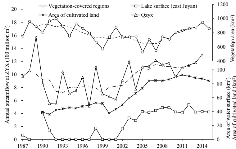
Figure 4. Temporal variations in river discharge at ZYX (triangle), annual total vegetation-covered regions (circle), East Juyan Lake surface area (square) and cultivated lands (cross) from 1987 to 2015. The dash line and dash-dot line denote the 5-year moving average values for vegetation areas and streamflow at ZYX respectively.
