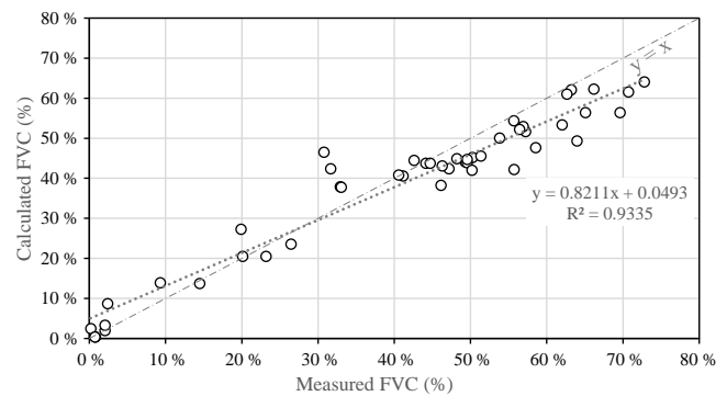
Figure 2. Comparison between the calculated and measured FVC values in 54 sites within HRB in 2014.
