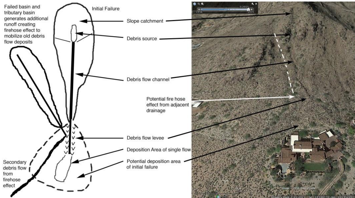
Fig 10. Idealized concept of debris-flow generation by two different processes in small arid basins of the Sonoran Desert. Field observations from the 2014 debris flow events at South Mountain indicate that failures high up on the steeper slopes of small drainages (Initial Failure) occur from high intensity precipitation events. This initial failure and also erosion associated with flooding in a tributary basin can set up conditions for subsequent debris flows from a firehose effect. The cleaned-out debris-flow chutes and tributary channels can end up funneling water efficiently to older debris-flow deposits. This process could potentially occur above home sites like this one. Mobilization of these older deposits can allow debris flows to extend farther down the piedmont than initial failures — as seen for the Elliot4 (Fig. 6) and Elliot6 debris flows on 8 September (Table 2).
