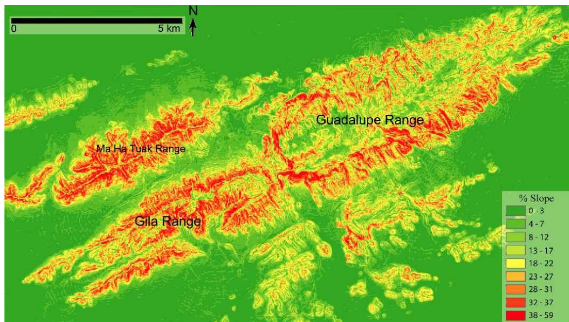
Fig. 3. Debris-flow chutes and levees occur on the steepest slopes of the Ma Ha Tuak and Gila ranges of South Mountain that experienced debris flows in 2014.
