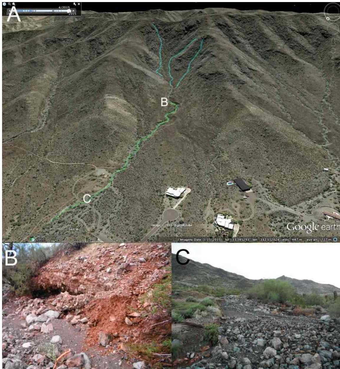
Fig. 6. Debris flows near Elliot Drive, Phoenix, failed in two different storms. (A) Blue lines denote Elliot flows 1-3 ( Table 1 ) that failed 12 August, while the green line indicates Elliot flow 4 that failed 8 September. (B) Photograph taken August 12 of saturated bank composed of late Pleistocene debris-flow deposits. This bank experienced a firehose effect on 8 September. (C) The 8 September debris-flow deposit generated by the firehose effect of runoff aimed at steep banks of older debris-flow deposits. Locations of the photographs (B) and (C) are indicated in (A)
