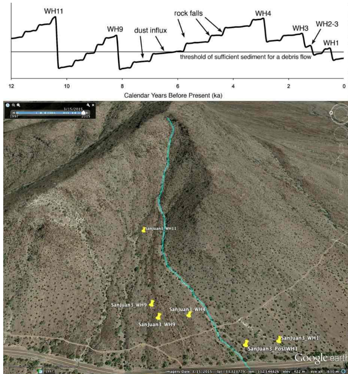
Fig. 9. A conceptual model for debris-flow chute rearming under present-day conditions in the Sonoran Desert, where the vertical axis in the graph indicates the amount of colluvium and fines accumulated in a debris-flow chute. The conceptual graph also refers to specific VML ages for debris-flow levees sampled adjacent to the San Juan 2014 debris flow indicated by the line. Pins indicate the sampling location for debris-flow levees of various Holocene ages ( Table 2 ). The model of re-arming desert slopes without climatic change is only conceptual because rates of dust influx, rates of rock fall influx, and threshold of sufficient sediment to generate a debris flow are unknown at present.
