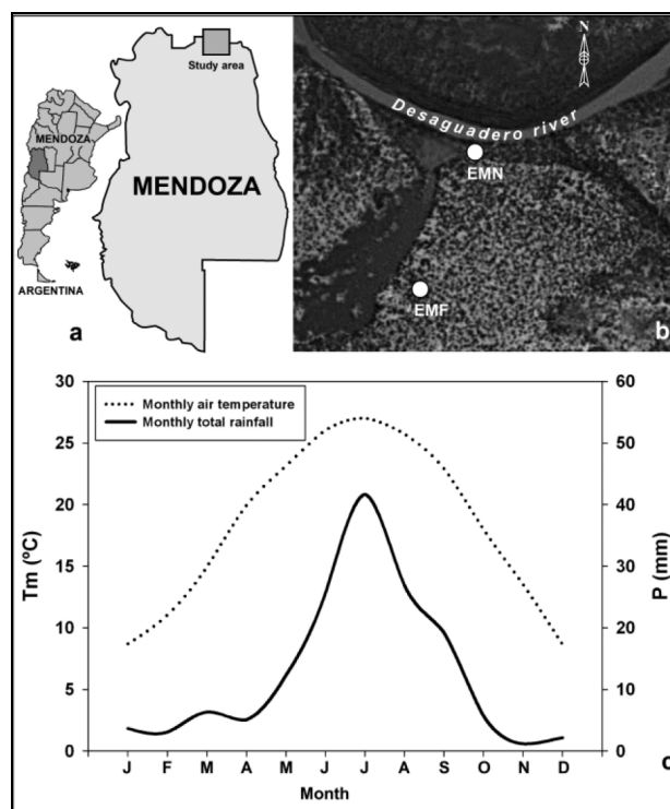
Fig. 1. Geographical location of the study area (a), spatial position of the sampled plots (b), and Ombrothermic diagram drawn according to the methods of Bagnouls and Gaussen (1953) (c). Precipitation and temperature data belongs to the Encón climatic station (32° 15' S, 67° 47' W), covering the 1971–1987 period. Source for the satellite images was Google Earth http://earth.google.es .
