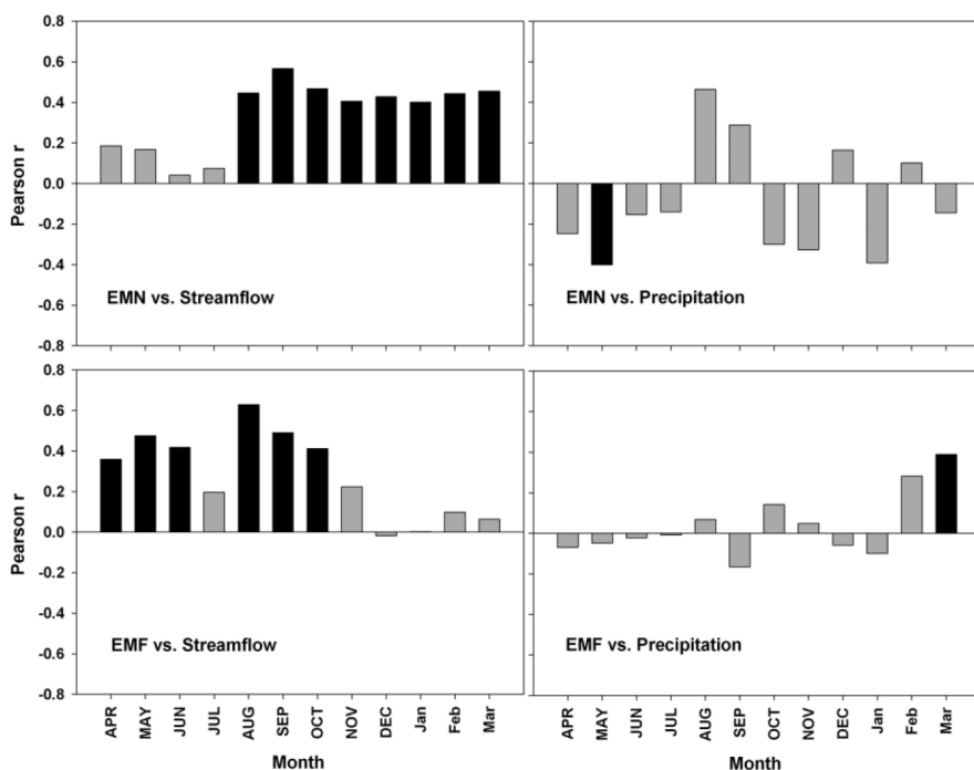
Fig. 4. Correlation functions between each EMN and EMF residual chronologies and monthly total streamflow and precipitation data for the common period 1991–2008. Black bars indicate significance at p < 0.05 .
