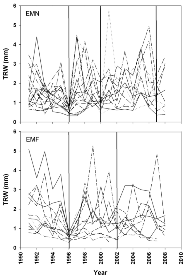
Fig. 3. Raw ring-width series of the analyzed trees showing pointer years (vertical lines) at the EMN and EMF plots for the common period 1991–2008.
