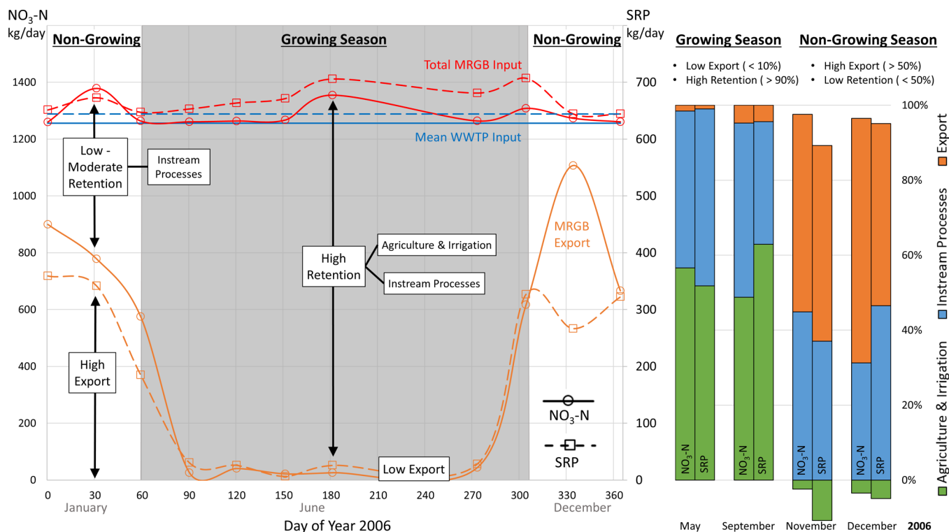
Figure 4. (Left) Aquatic nutrient inputs, retention, and export from the Rio Grande in the Middle Rio Grande basin during 2006. \text{NO}_3\text{-N} is shown by continuous lines and circles using the left axis; SRP is shown by dashed lines and squares using the right axis. (Right) Nutrient loading partitioned between agriculture, instream processes, and export for growing season (May, September 2006) and nongrowing season months (November, December, 2006). Partitioning is expressed as percentages of total loading for \text{NO}_3\text{-N} (left columns) and SRP (right columns).
