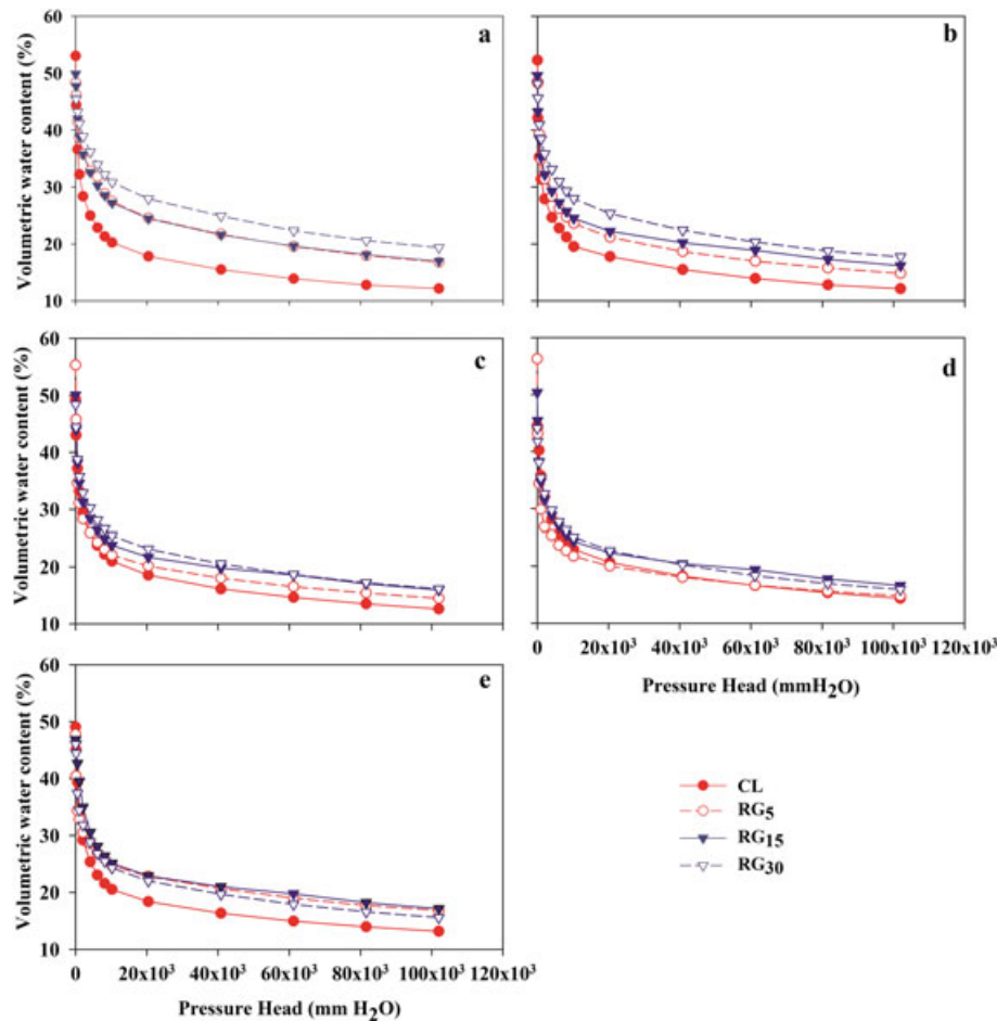
Figure 4. Soil–water characteristic curves for a soil under four treatments (cropland, CL, and restored grassland, RG, where subscripts indicate the restoration age in years) for five soil depths (a, 0–5 cm; b, 5–10 cm; c, 10–20 cm; d, 20–30 cm; e, 30–50 cm).
