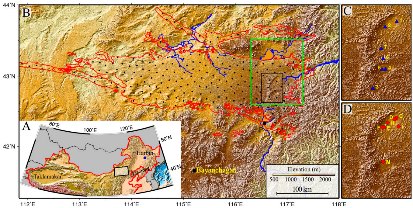
Fig. 1. Geographical location of the Hunshandake Sandy Lands (A) and its area (encircled by red line in B). The black rectangle in B marks the location of the enlarged maps C and D on the Right, and the green rectangle shows the location of Fig. 2. Map C shows the localities of water samples, and map D shows the localities of sections with stratigraphy presented in Fig. 3. The sand–paleosol section P (Fig. 3) is on the southern margin, and the site Bayanchagan marks the coring site of ref. 8. Rivers with headwaters in the Hunshandake likely formed by groundwater sapping are marked in blue. Drainages to the southwest and west are currently undergoing groundwater sapping, with substantial spring-driven flow found at the current river base level.
