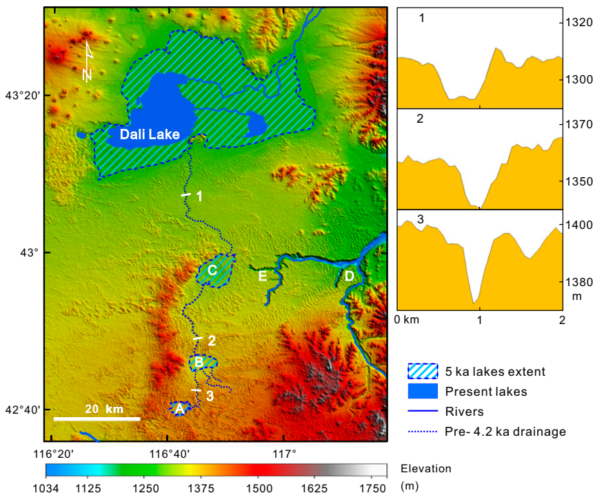
Fig. 2. (Left) Holocene lakes and channels in the Hunshandake and lake extent at selected epochs. Upper, middle, and lower lakes are indicated by points A, B, and C, respectively. Xilamulun River (point D) drains to the east. Groundwater-sapping headcuts at the upper reaches of incised canyons (point E) suggest a mid-Holocene interval of easterly surface flow, followed by groundwater drainage beginning at the ca. 4.2 ka event. Northern and central channels at point E are currently abandoned, and groundwater sapping has migrated to the southerly of the three channels shown. (Right) Cross-sections of the predrainage shift, northerly drainage into Dali Lake (Localities shown on the Left), showing the increase in widths of channels downstream (Vertical exaggeration \sim 30:1 ).
