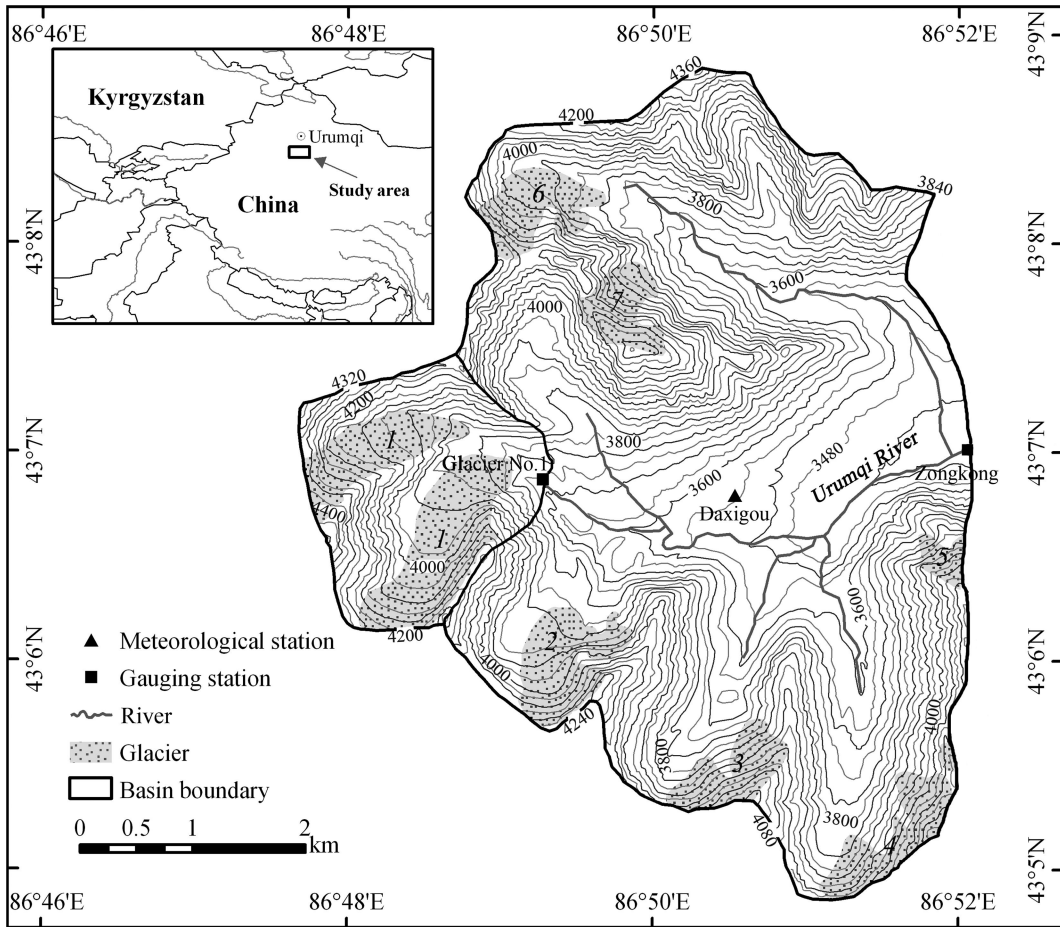
Fig. 1. Map of the Ürumqi river source region showing the locations of glaciers and hydrological and meteorological stations.
