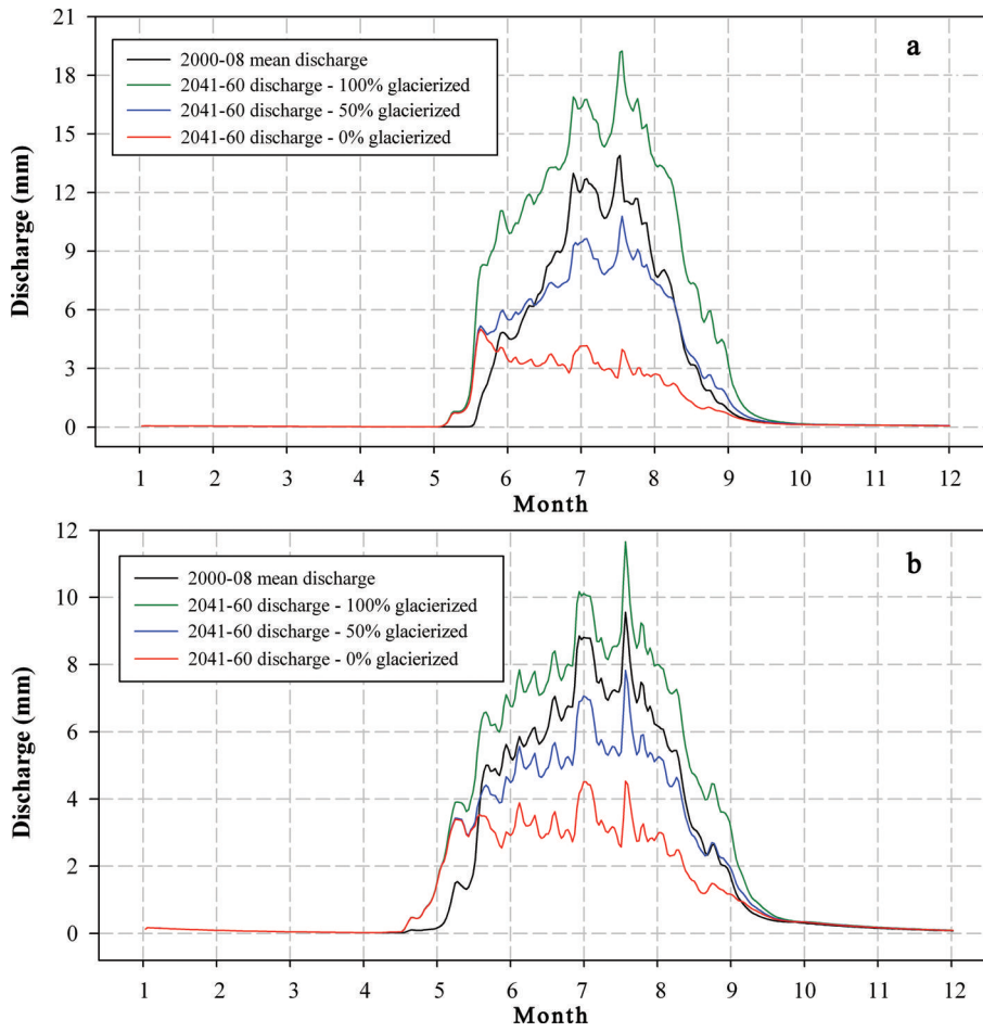
Fig. 6. Annual discharge cycle of (a) Ürumqi glacier No. 1 and (b) Zongkong catchments simulated by HBV for current climate (2000–08) and future climate (2041–60) for three stages of glaciation.
