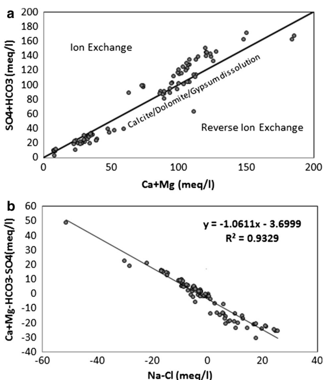
Fig. 4 a SO_4+HCO_3 versus Ca+Mg plot. b Ca+Mg-HCO_3-SO_4 versus Na-Cl plot
