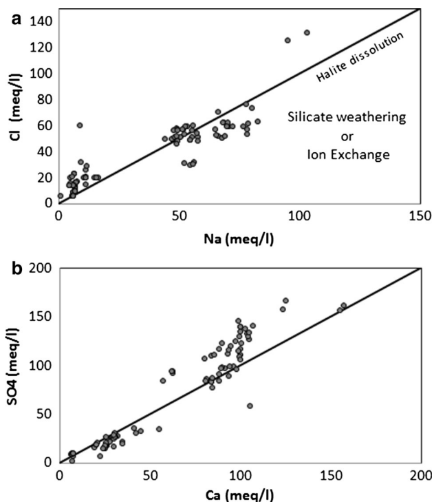
Fig. 5 a Cl versus Na plot. b SO_4 versus Ca plot
