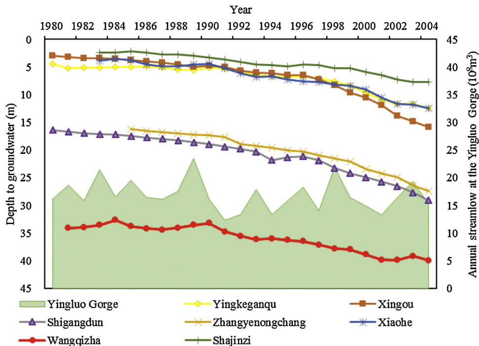
Fig. 4. Annual depth to groundwater at 7 monitoring stations in the Ganzhou district, and the annual streamflow at the Yingluo Gorge (upstream).
