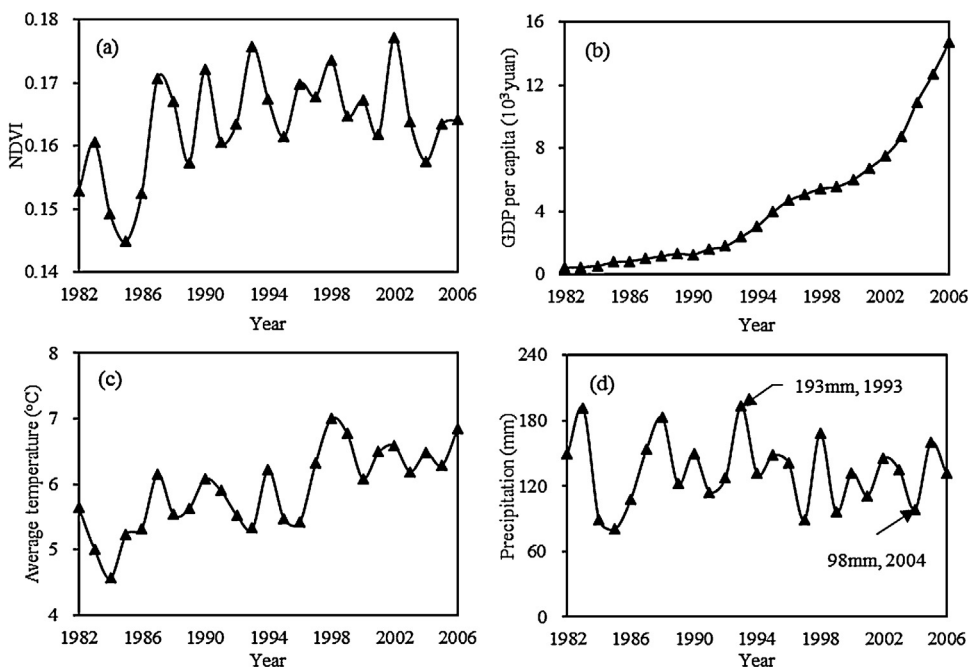
Fig. 10. Time series of the NDVI, GDP per capita, average temperature and precipitation in the middle Heihe River Basin from 1982 to 2006.
