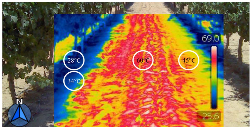
Figure 6. RGB image with overlaid thermal image of the vineyard inter-row that were acquired simultaneously on 23 July 2012 at 12:35. The legend refers to temperature ( ^{\circ}\text{C} ) and circled numbers represent average temperatures for respective surfaces.
