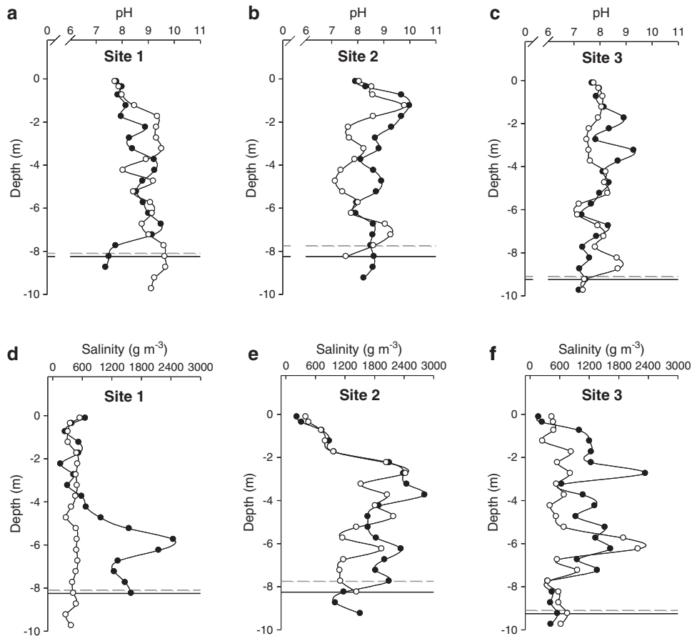
Figure 4. Vertical distribution of soil pH (a–c) and salt content per metre cubic of soil (d–f) in control woodlands (filled circles) and livestock stations (open circles). Each symbol represents a single measurement. The horizontal solid and dotted lines indicate the water table level for control woodlands and livestock stations, respectively.
