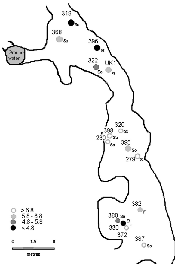
Fig. 6. Spatial distribution of Site 2 water isotope samples: see inset, Fig. 1 for location within Cathedral Cave. Site ID and drip classification are as presented in Table 1. Shading and fill of the symbols shows the slope of \delta^2\text{H} vs. \delta^{18}\text{O} regression as presented in Table 1.
