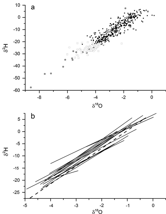
Fig. 4. (a) \delta^2\text{H} vs. \delta^{18}\text{O} for monthly rainfall (closed circles) and infiltration (small closed squares). Local river water samples (open squares) and groundwater samples (open circles) are also presented. (b) Trend lines of the data presented in (a): Local Meteoric Water Line (dashed line) and \delta^2\text{H} vs. \delta^{18}\text{O} regressions for each drip water site (solid lines). Regression equations and correlation coefficients are presented in Table 1.
