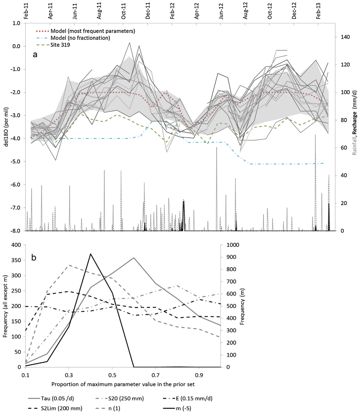
Fig. 7. (a) Results from Monte Carlo modelling of drip water compositions shown against observations (solid lines, except dashed Site 319), and observed rainfall and modelled groundwater potential recharge. Shaded area represents the isotopic distribution of the physically plausible model results (1927 out of 50 000). The model output for the most frequently used parameter values are highlighted (dots) and for no karst evaporation/fractionation (dash-dotted) (b) Frequency distributions of the posterior parameter sets, normalised across the range of prior parameter values. Each parameter was free to vary between zero and the value defined in brackets. For example, m was free to vary randomly between 0 and -5 but most models that had a reasonable fit have values of around -2 . The parameters are the recession constant, the initial value of store S2, evaporative flux from store S2, the S2 store threshold for evaporative fractionation to occur, the empirical constants n , the empirical constant m .
