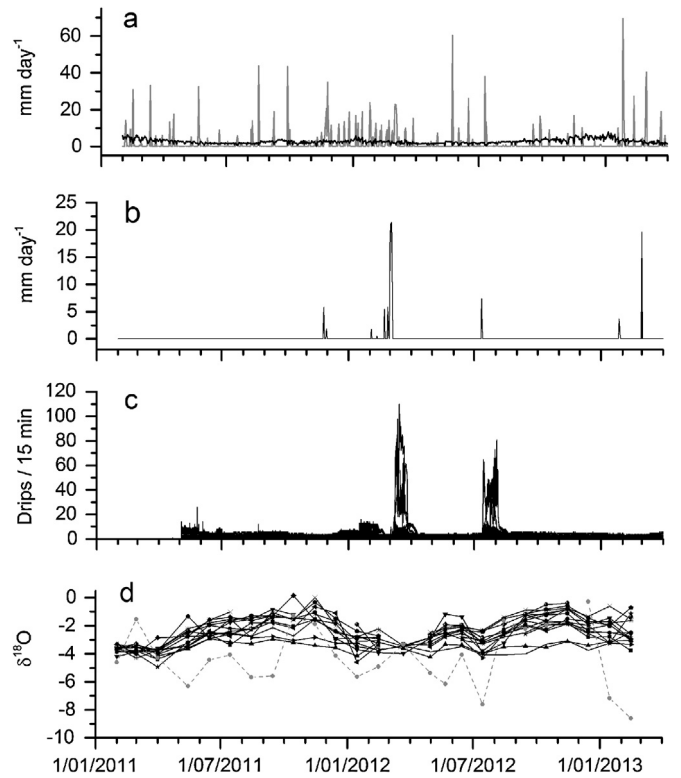
Fig. 3. (a) Rainfall (grey line) and potential evaporation (black line); (b) modelled groundwater potential recharge; (c) drip rate for all Stalagmate drip loggers over the study period; (d) rainfall (dashed line) and drip water (solid line) monthly isotope samples.
