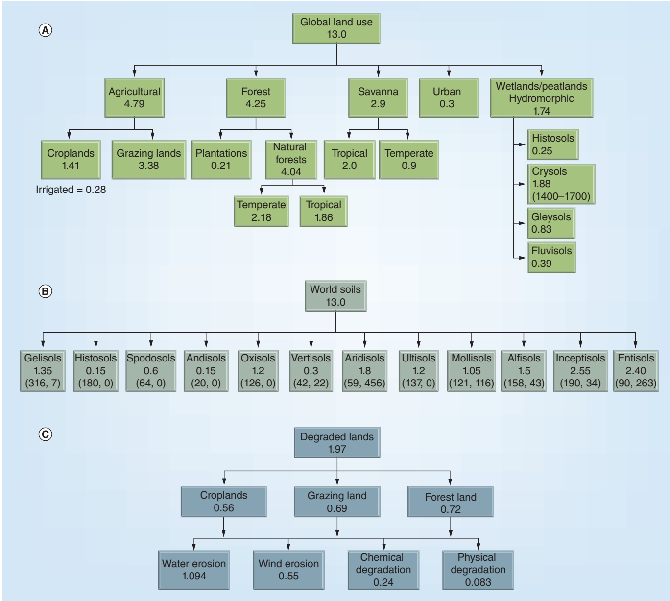
Figure 9. Global estimates of land use, soil resources and the state of their degradation by different processes. (A) Estimates of land area are 109 ha under different ecosystems. Data on land area taken from [60,169,173,306]. (B) Estimates of area in 109 ha under different world soil orders (data on area are from [244]) and of the magnitude of carbon pool to 1-m depth in Pg shown in parenthesis (soil organic carbon, soil inorganic carbon) are from [245]. Data on soil organic carbon pool in Cryosols taken from [60]. (C) Estimates of areas affected by soil degradation under different land uses and by different processes are from [246]. The sum of the individual land use area may exceed the total because of overlaps and duplications.
