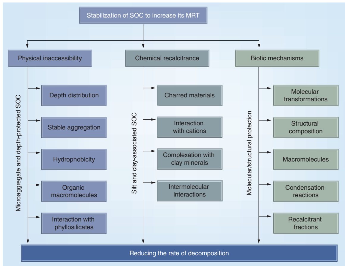
Figure 3. Mechanisms of stabilization of soil organic matter.
