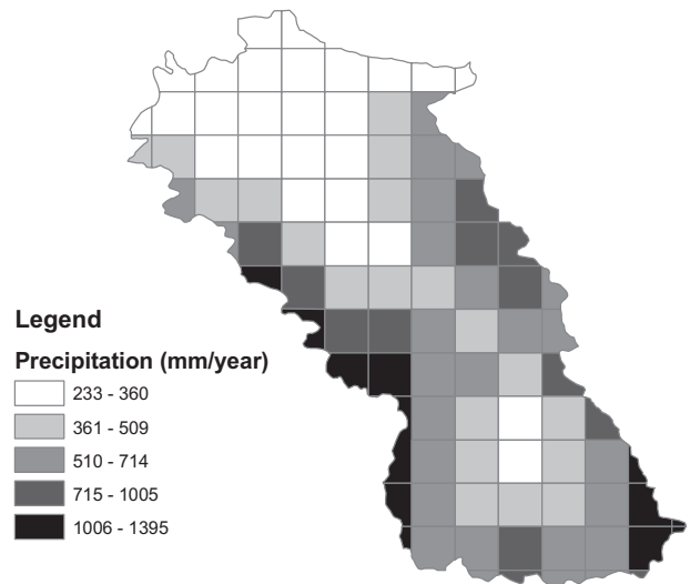
Fig. 4. Spatial distribution of average annual precipitation (mm/year) during the period of 1990–1999 for the North Platte River watershed.
