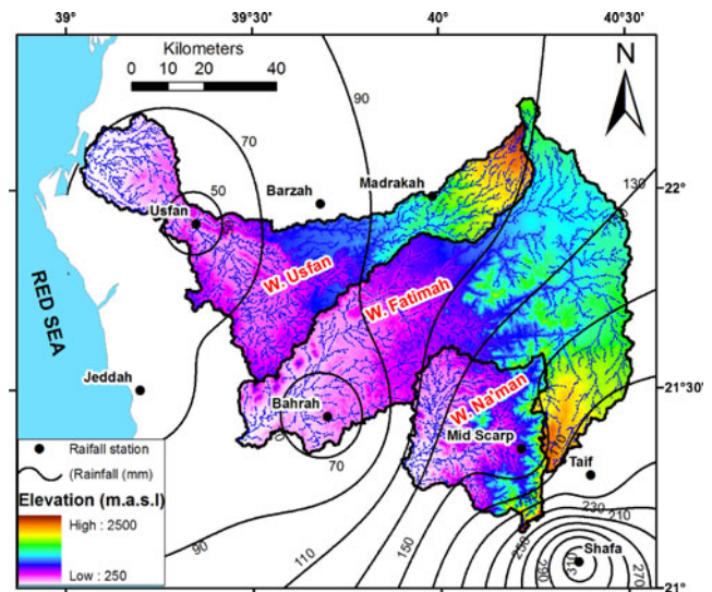
Fig. 1 Map showing the isohyetal lines of annual rainfall and main basins in the study area
