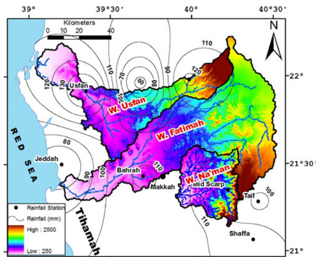
Fig. 4 Annual maximum observed of 24-h rainfall
